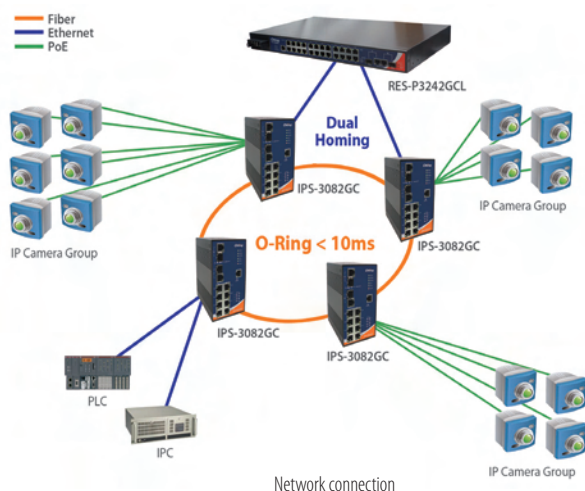
Network connection
